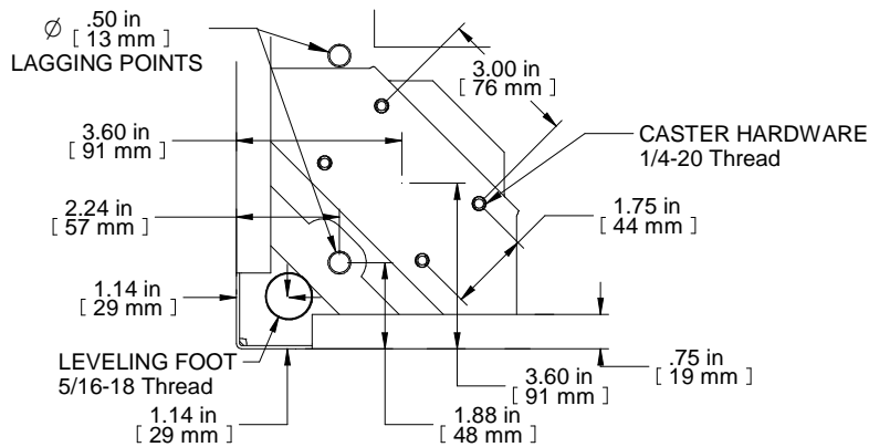
DETAIL A 4X SCALE 5:1
